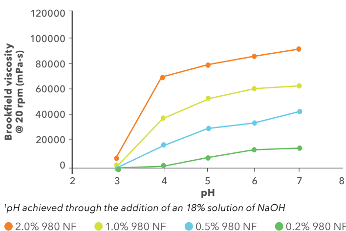
Figure 2. Effect of pH and Concentration on the Viscosity of Carbopol 980 NF Polymer Dispersion 1
