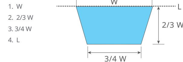
Figure 1: Relative Dimensions of a Trapezoidal Runner for use in a Three-plate Mold
