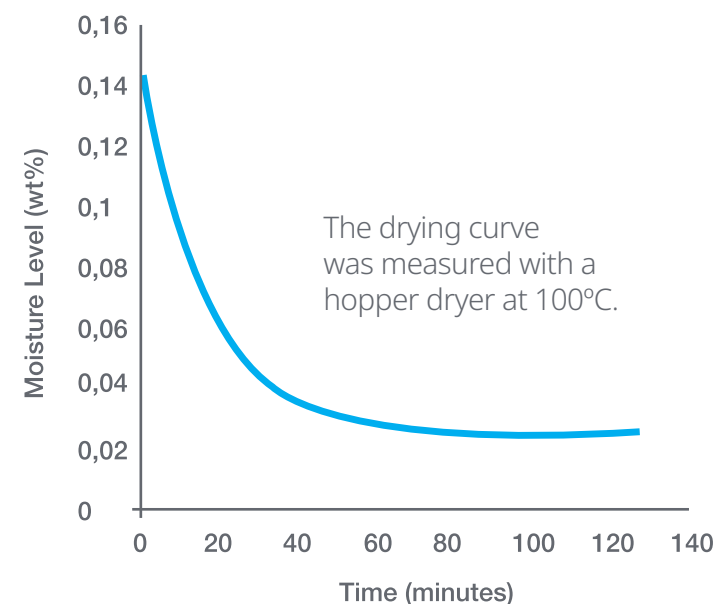
Figure 6: Drying and Moisture Absorption curves
