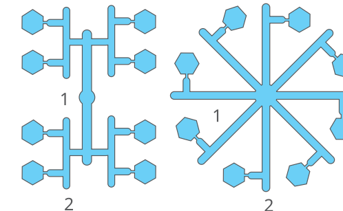
Figure 3: Runner Systems with balanced-flow Cavity Layouts and Cold Slug wells
